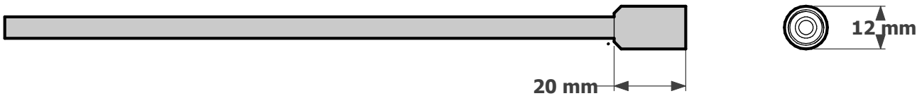
6mm diameter rod with a M10 x 1P Internal thread attached
