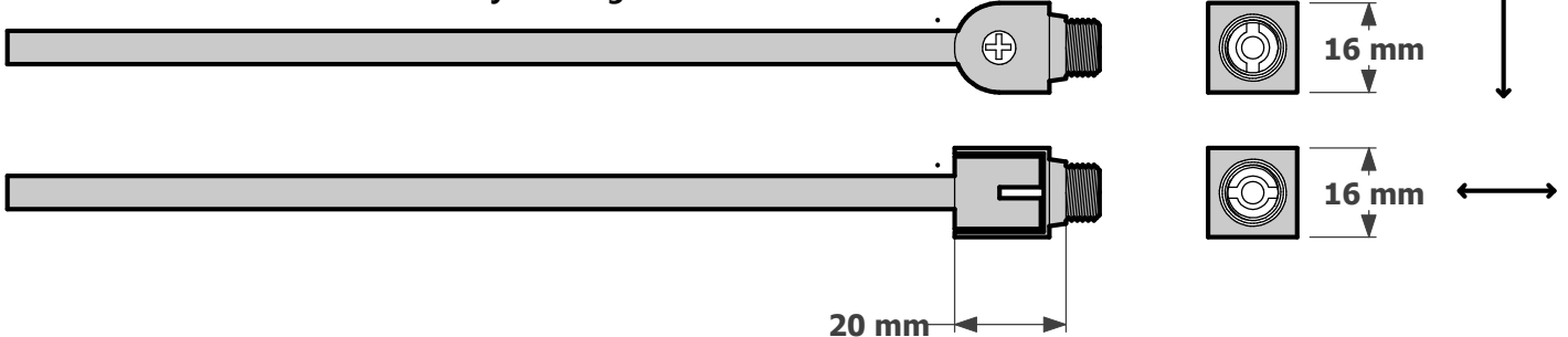
6mm diameter rod with a one way 180 degree swivel attached
