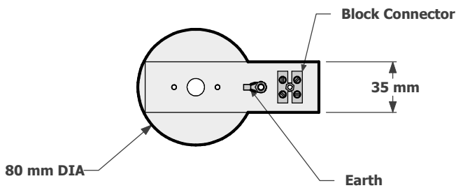
Suits 65mm DIA cut out
